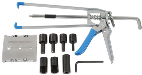
Pipe Connector Insertion Tool | 6933
